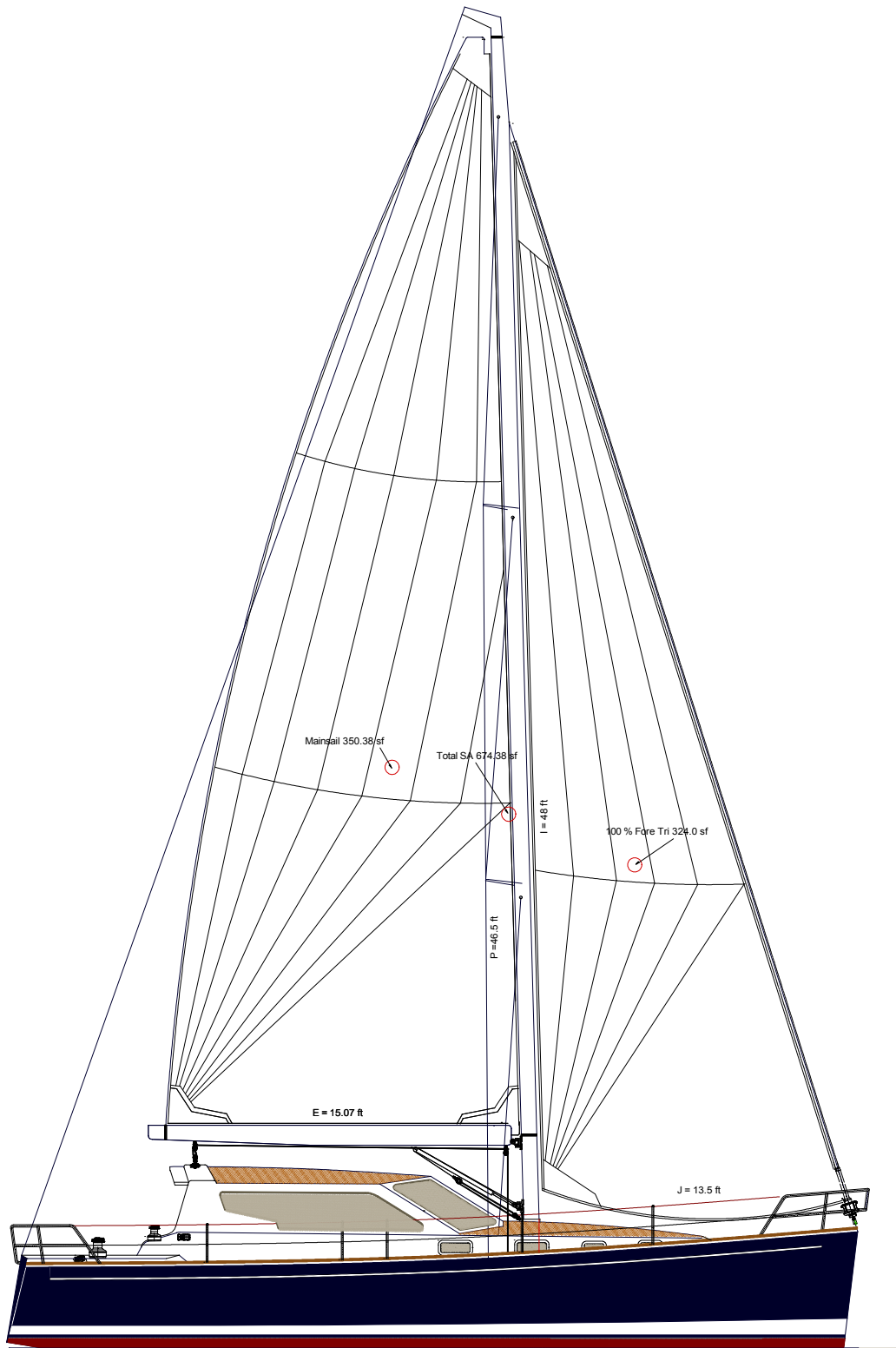
SAIL PLAN
